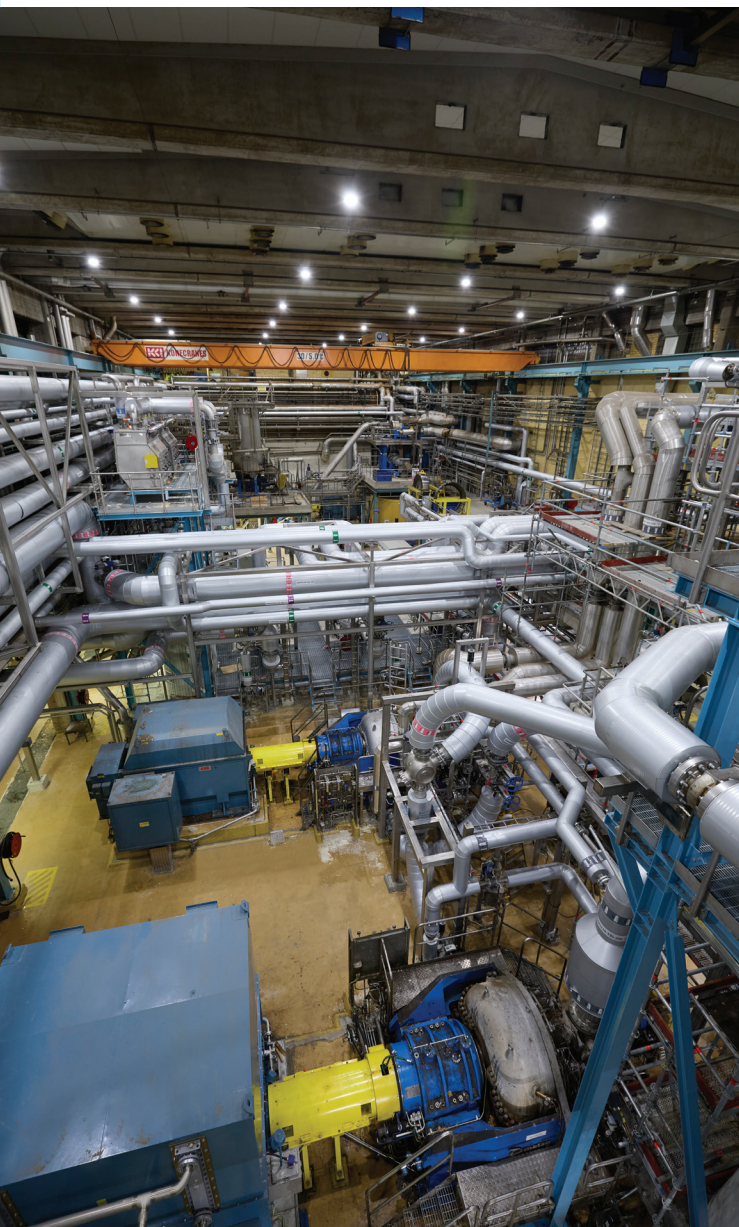
Figure 4: Primary and secondary refiners.
