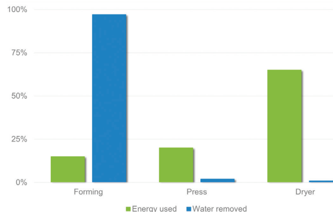
Figure 1: Comparison of the press section with the forming and drying sections concerning overall water removed and energy used [3].
