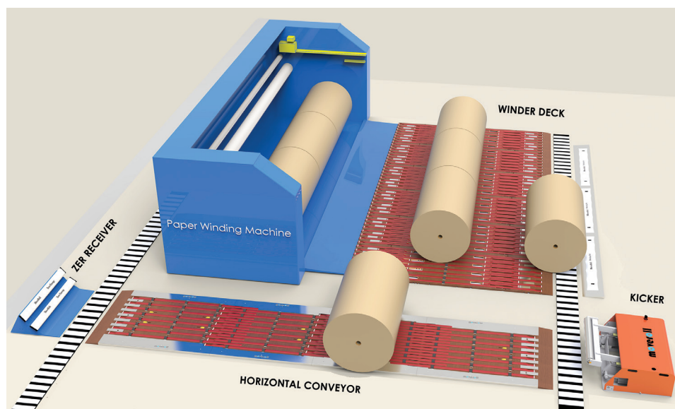
Figure 7: Winder deck.
