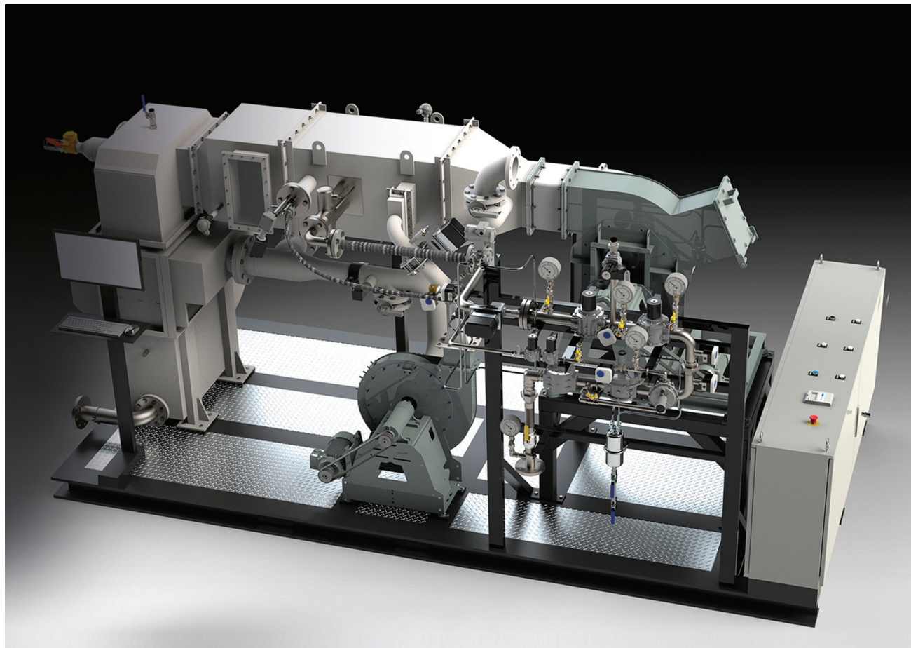
Figure 6: Toscotec's TT Hydrogen Burner.
