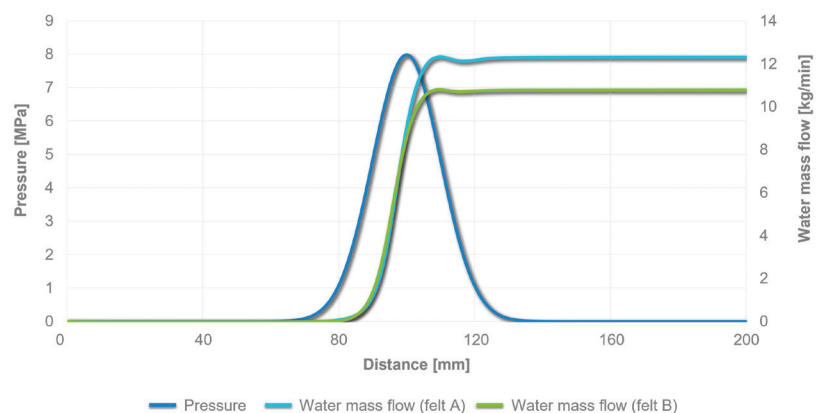
Figure 7: Results from the process simulation: Pressure profile and dewatering behavior of two different press fabrics in a roll press nip.
