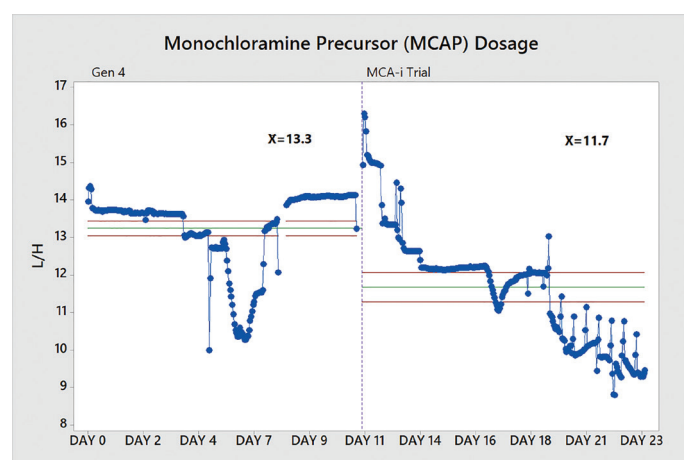
Figure 2: Phase 1 Trial Evaluation of MCAP and Sodium Hypochlorite Dosage Rates. For the MCA-i trial, both chemical flow rates were reduced while maintaining a slightly higher headbox MCA residual (Figure 1) as compared with the Gen 4.
