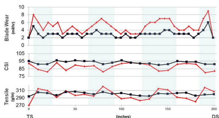
Figure 7: Cross directional profile on a CWP machine showing blade wear (mils/hr), crepe structures per inch (CSI), and tensile strength (g/in) for TULIP™ (in blue) vs. a conventional PAE (in red). The light-blue shaded columns in the CD represent areas of higher sheet moisture coming to the Yankee and hence areas subjected to potential durability issues for the coating. On the x-axis TS and DS represent the tending and drive sides of the machine, respectively.
